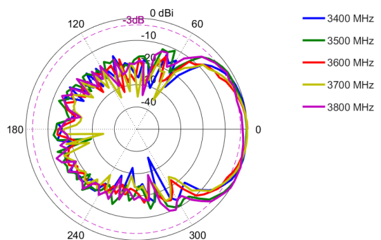
Elevation: 3400 – 3800 MHz
